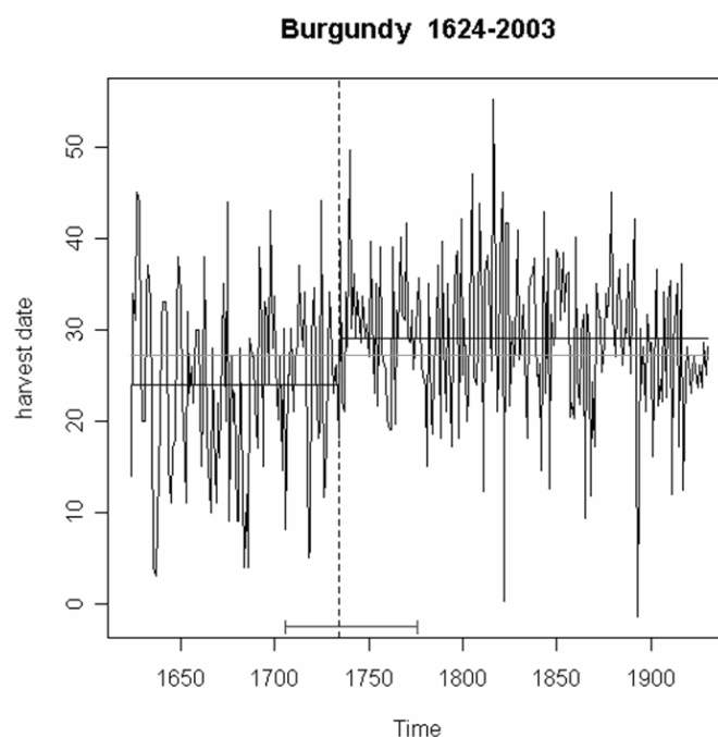
Fig. 7 - Diagram showing the result of the breakpoint analysis carried out on harvest data of Burgundy (Chuine, 2004). The most probable year of discontinuity is 1734 (vertical line) and with a confidence of 95% the discontinuity drops into the range 1706-1776 (horizontal range). The mean harvest date is 24 before the discontinuity and 29 after.
