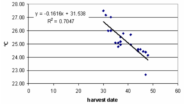
Fig. 3 - Scatterplot showing the linear model (straight line) interpolating harvest dates (x) and May-June – July mean maximum temperatures (y).
