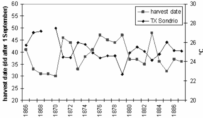
Fig. 2 – Temperatures of Sondrio and grape harvest dates of Tirano. The opposite correlation is evident.
