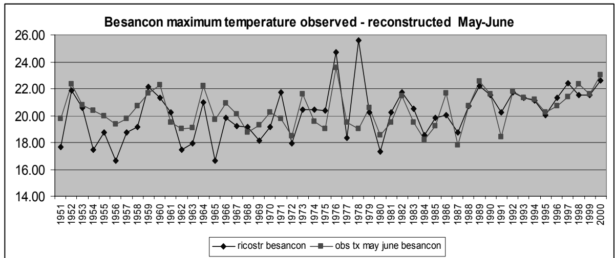
Fig. 5 – average maximum temperatures of May – June for Besancon: comparison between measurements at Besancon airport and simulations carried out applying LM1 to harvest data collected by Chuine et al. (2004)
