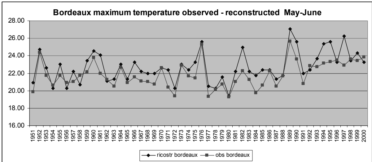
Fig. 4 – Average maximum temperatures of May – June for Bordeaux: comparison between measurements at Bordeaux Merignac airport and simulations carried out applying LM1 to harvest data collected by Chevet (2006)
