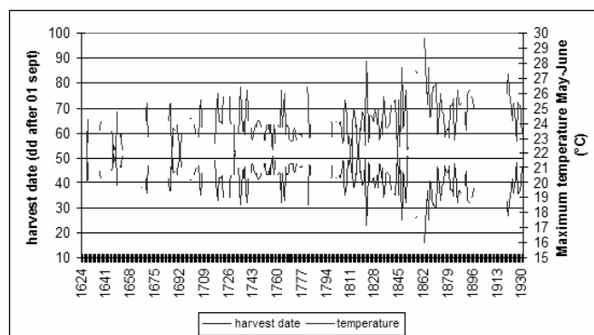
Fig. 6 - Temperature reconstruction for Valtellina (MAY- JUNE) from available harvest dates from Zoia (2004)
