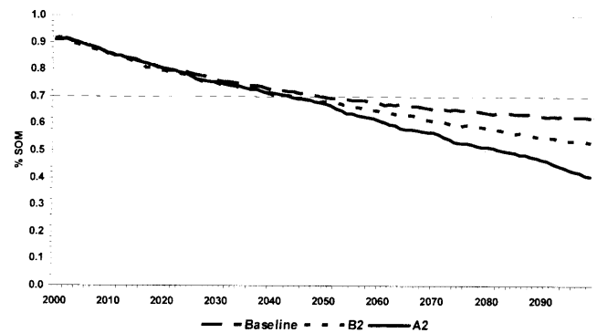
Fig. 4 - Soil carbon dynamic simulated by CropSyst as influenced by transient climatic scenarios.
