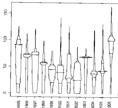
Fig. 6 - Box-percentile plots of date (day of the year) of the last late frost for the 90 stations available on Ucea web site (horizontal lines represent maximum, upper quartile, median, lower quartile and minimum; for more information about the meaning of this kind of plot see Easy and Bafield, 2003). A progressive delay of the last frost can be observed in the last years.
