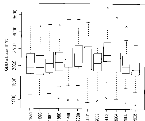
Fig. 5 - Boxplots of yearly growing degree days cumulated on the base temperature of 10°C from the daily data of 90 stations available on Ucea web site (each boxplot represents maximum, upper quartile, median, lower quartile and minimum; outliers are excluded from calculations and represented with circles). A gradual decrease is evident after the high values attained in 2003.
